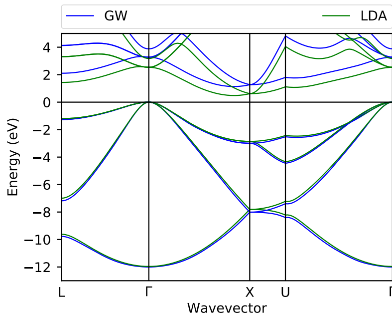
Fig. 2 Shown are the band structures of silicon at the LDA and GW computed by BerkeleyGW in this exercise.
