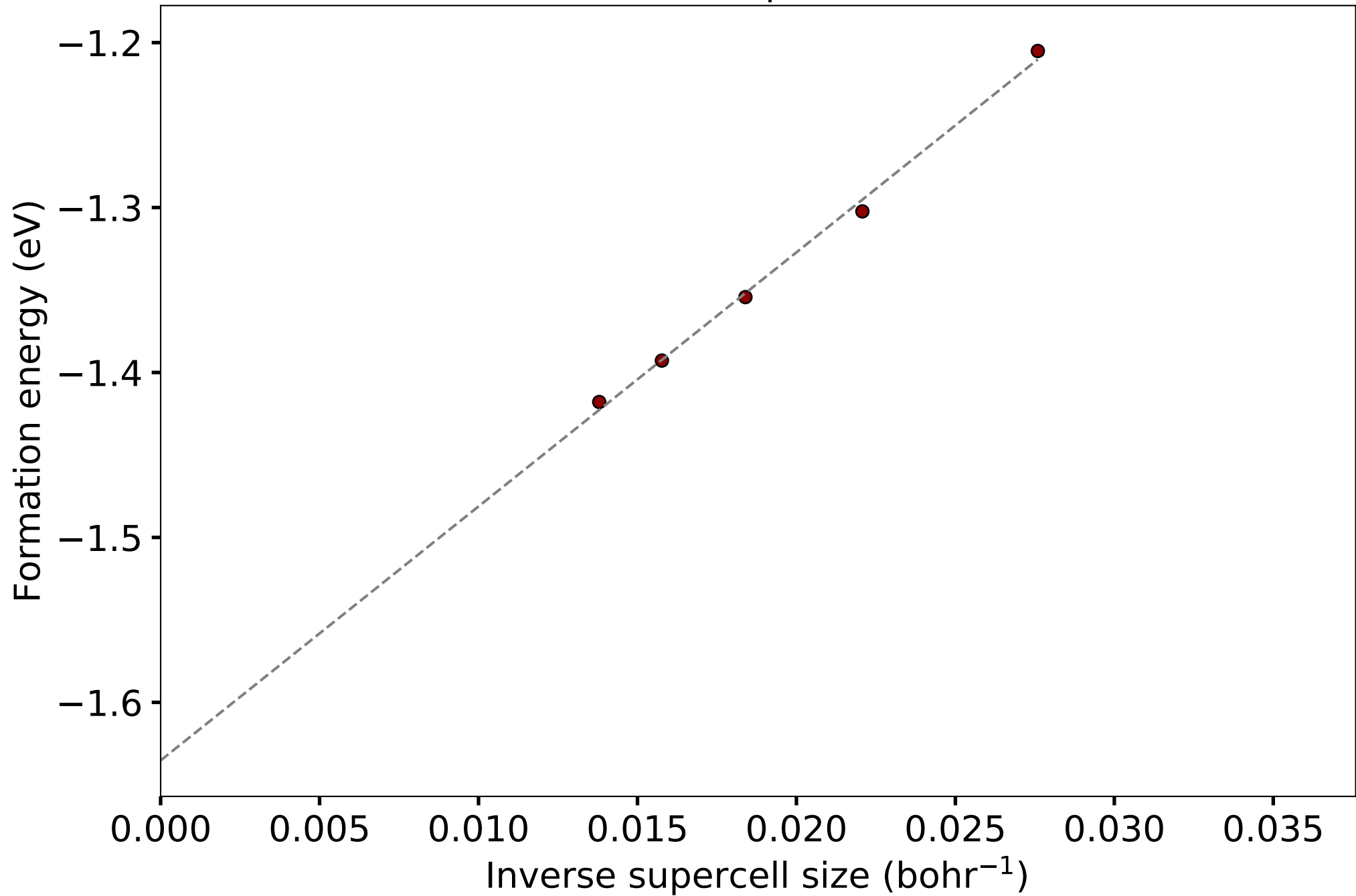
LiF hole polaron
